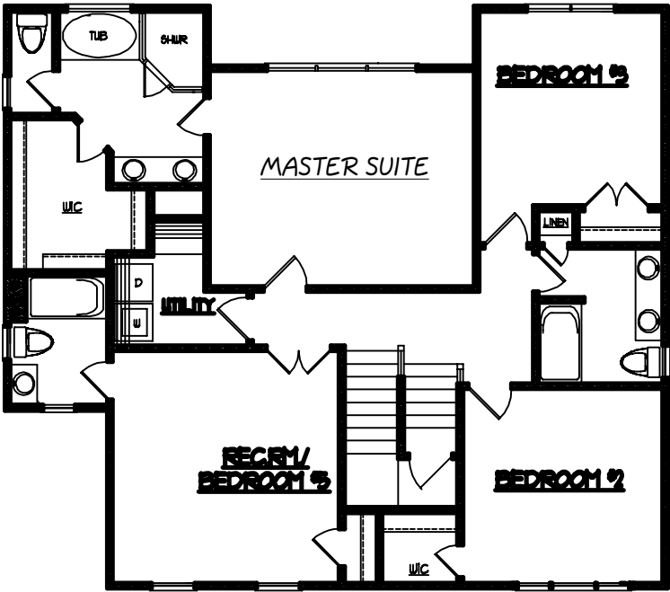
SECOND FLOOR
