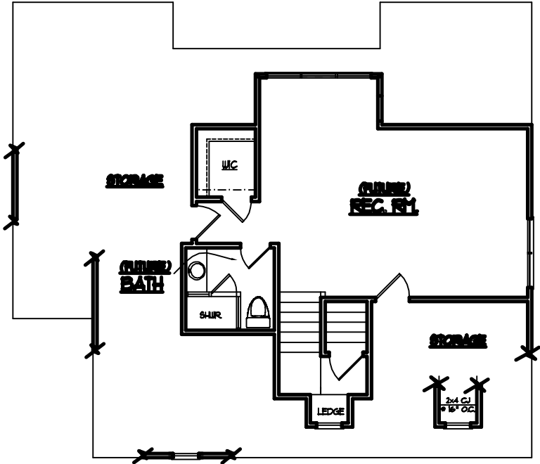
THIRD FLOOR
